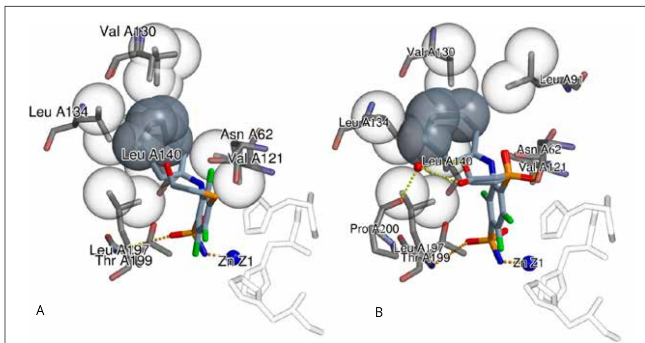
Figure 2. Compounds 1 (Panel A, PDB ID 4Q06) and 3 (Panel B, PDB ID 4Q07) bound to chCA IX as determined by X-ray crystallography. The Zn is shown as a blue sphere, while the histidine residues holding the Zn atom are transparent. The amino acids of chCA IX are shown in grey. The terminal atoms of amino acids which form the hydrophobic
