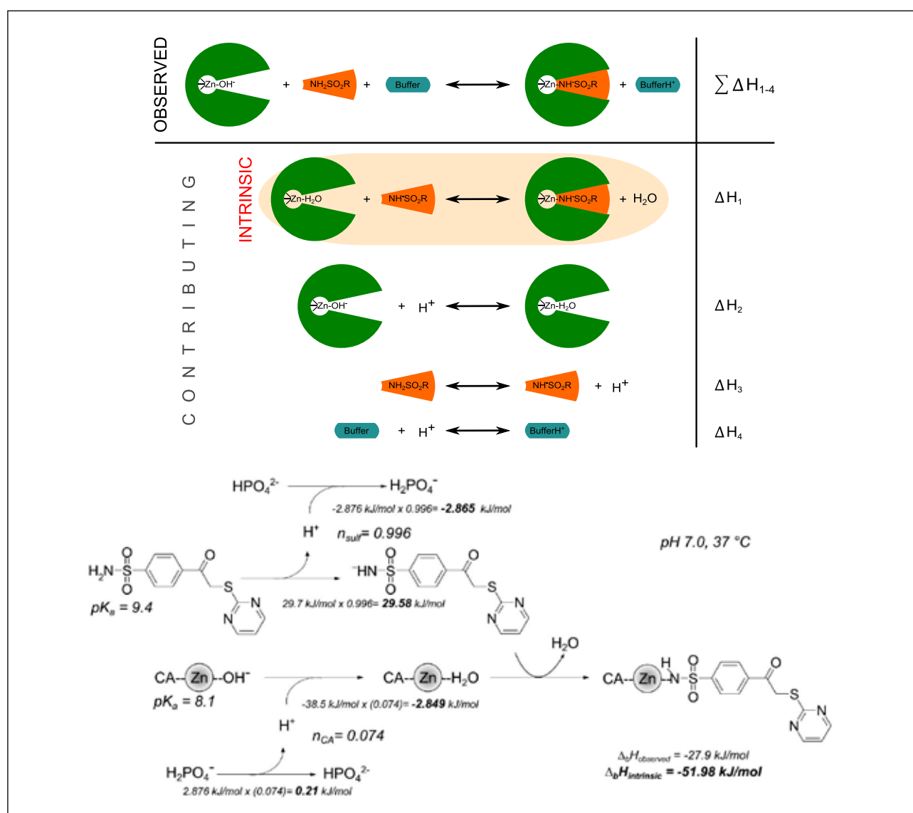
Figure 3. The observed and intrinsic binding thermodynamics. The upper panel shows the main linked reactions occurring upon ligand binding to CAs. The lower panel lists the enthalpies of all processes linked to the binding of 3b to CA I. The two left-central reactions show the binding-linked deprotonation of the inhibitor sulfonamide and the protonation of the zinc-bound hydroxide, respectively. Top and bottom lines show linked phosphate buffer (de)protonation reactions. The numbers give
