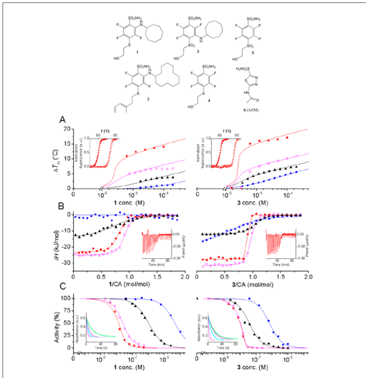
Figure 1. The top panel shows the chemical structures of CA inhibitors 1-6. Acetazolamide (6, AZM) is commonly used as a control inhibitor of CAs. Panels A, B and C show compound 1 (graphs on the left) and 3 (graphs on the right) binding and inhibition of CAs. A. Binding of compounds as determined by the thermal shift assay. Datapoints show the \Delta T_m s as a function of total added compound concentration while the lines are simulated according to 42 . Red filled squares – CA IX, magenta open squares – cbCA IX, black filled triangles – CA II, and blue filled circles – CA I. The largest \Delta T_m shift for similar proteins corresponds to strongest binding K_d . The inset graphs show normalized raw fluorescence data as a function of temperature at zero (filled red diamonds) and 50 \mu M (open red triangles) total added compound concentrations. The melting midpoints correspond to the T_m . B. Binding of the compounds as determined by the isothermal titration calorimetry. Colors and symbols for CA isoforms are same as in panel A. The ITC curve fitting K_d s are listed
