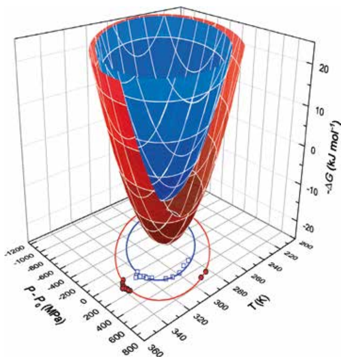
Figure 6. The Gibbs free energy dependence on pressure and temperature. Inner surface represents the ligand-free Hsp90N stability region, while outer surface shows stability region of protein-ligand system with 200 \mu\text{M} of added ligand [13].
