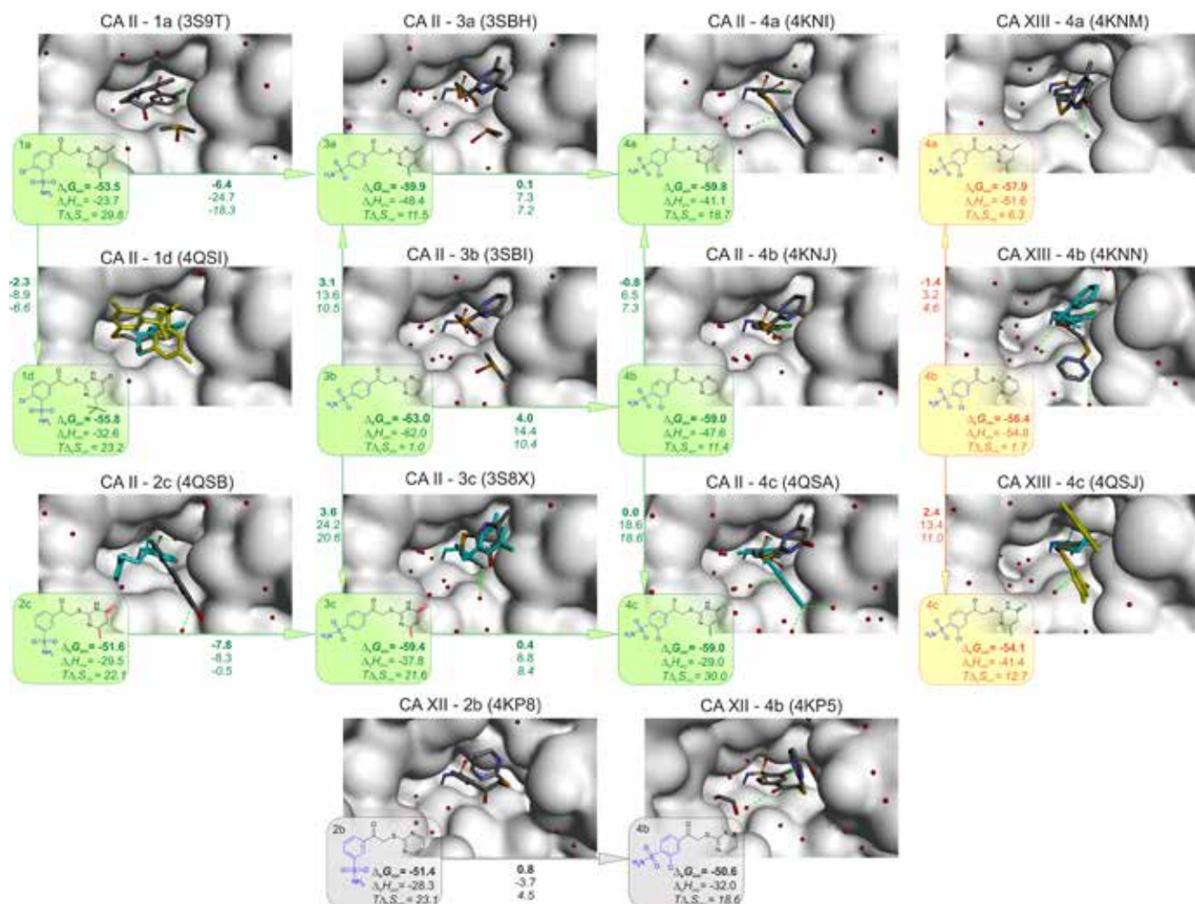
Figure 5. Compound chemical structure and the thermodynamics of binding correlations with the crystal structures of some compound binding mode in the active site of CAs (1a, 1d, 3a, 3b, 3c, 4a, 4b, and 4c with CAII; 4a, 4b, and 4c with CA XIII; 2b and 4b with CA XII). The thermodynamic parameters of binding and the colors of the shapes are same as in Figure 4 and indicate the CA isoform. Colors in the crystal structures are: yellow shows the pyrimidine ring that is not fixed in the crystal structure and has multiple conformations with low occupancies; blue shows the alternative conformation of the pyrimidine ring when both conformations are visible in the electron density maps.
